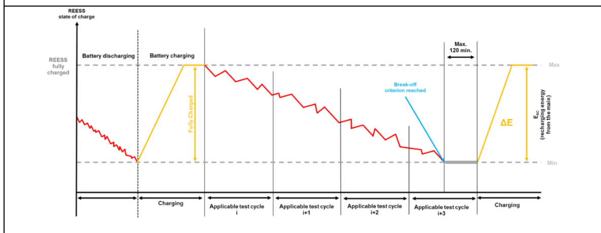
Figure A8.App1/6 Consecutive cycles test sequence PEV
