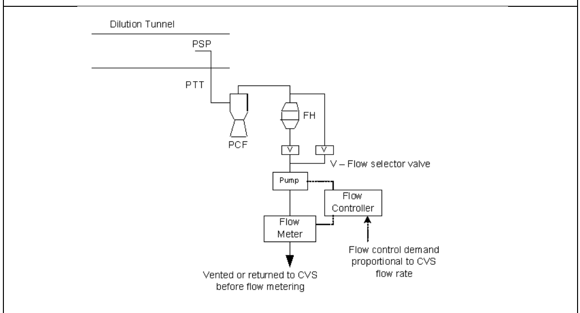
Figure A5/12 Particulate sampling system
