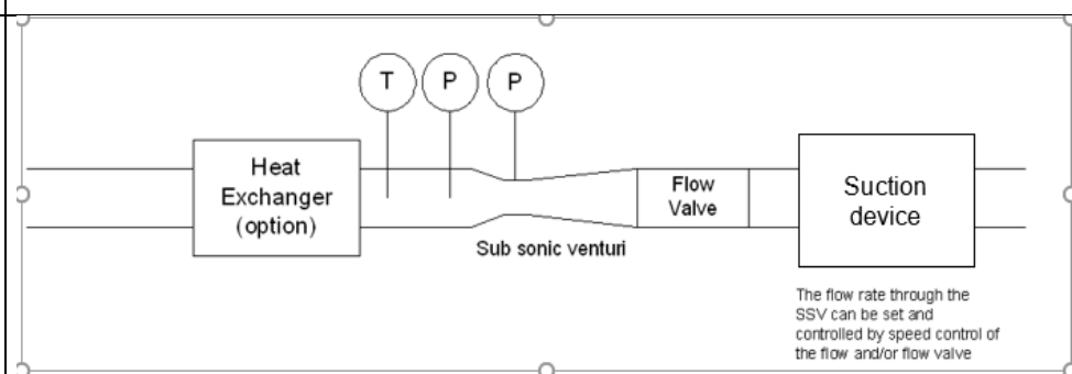
Schematic of a subsonic venturi tube (SSV)
