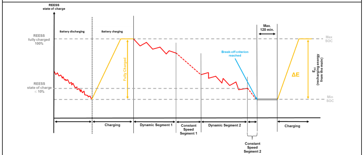
Figure A8.App1/7 Shortened test procedure test sequence for PEVs
